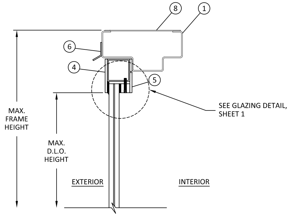
A 6 VERTICAL SECTION HEAD
