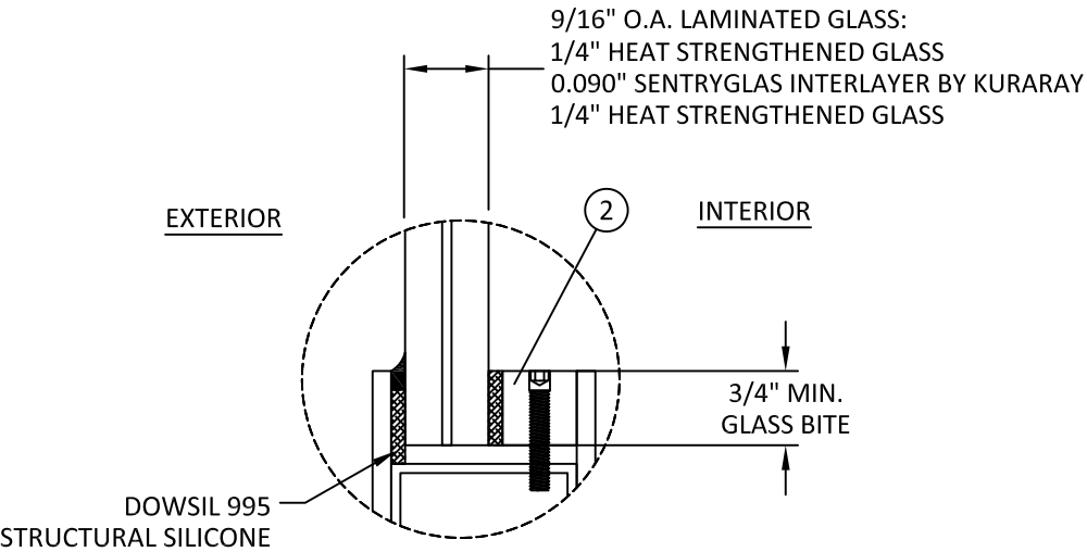
GLAZING DETAIL 1
