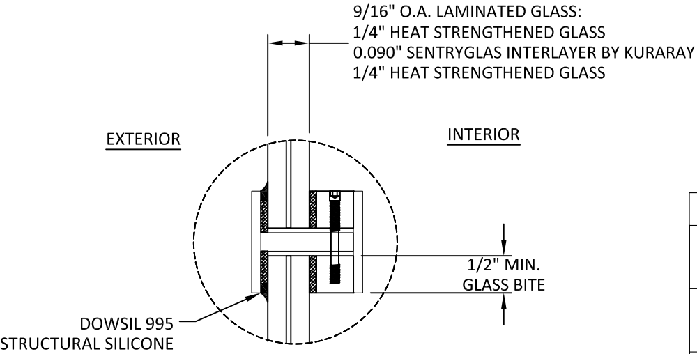
GLAZING DETAIL 2
