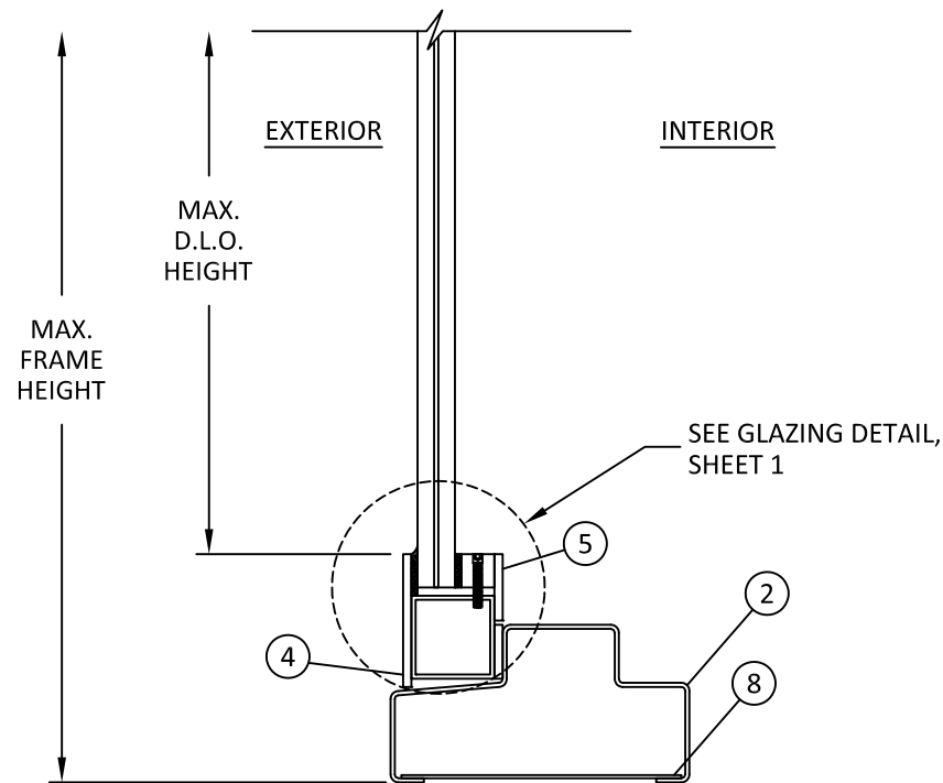
B 6 VERTICAL SECTION SILL
