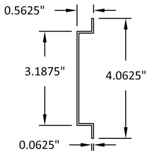
7 MULLION REINFORCEMENTS STEEL
