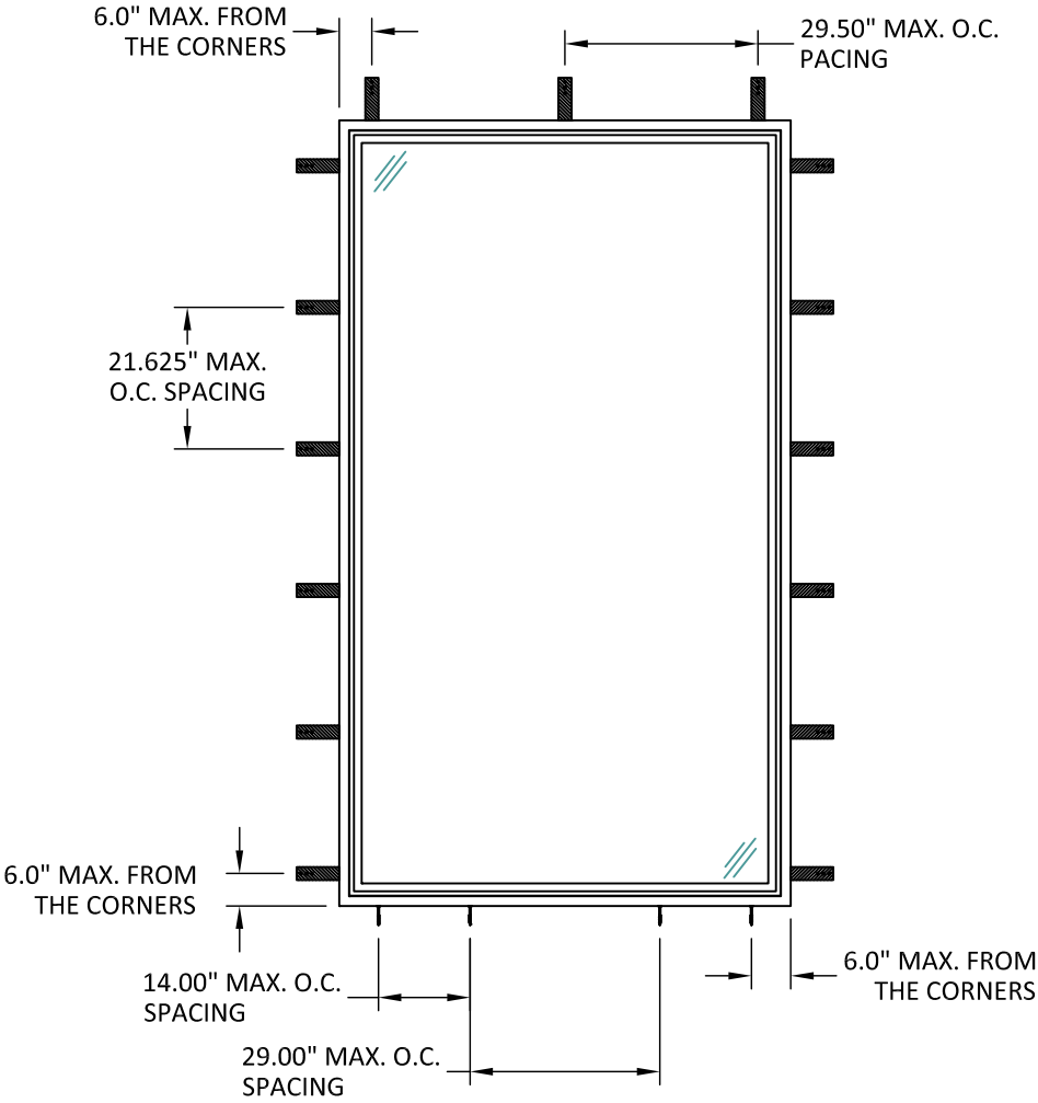
ANCHOR LAYOUT
