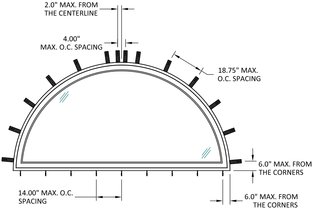
ANCHOR LAYOUT
