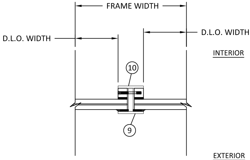
D HORIZONTAL SECTION 7 TYP. TDL
